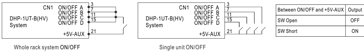
Figure 4-1 Connection of Remote Control
