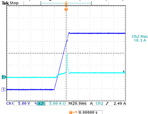
INPUT=24VDC @ FULL LOAD
