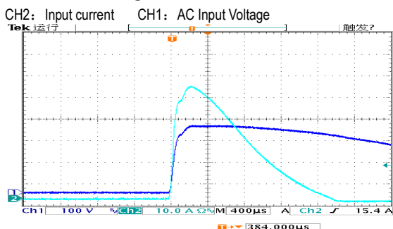
INPUT=230VAC/50HZ @ FULL LOAD
