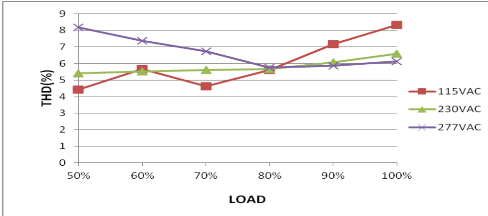
THD vs LOAD
